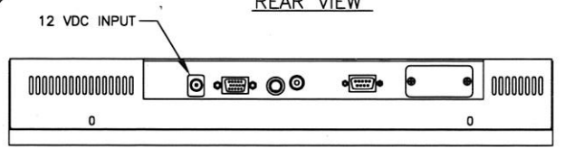
CONNECTOR VIEW
